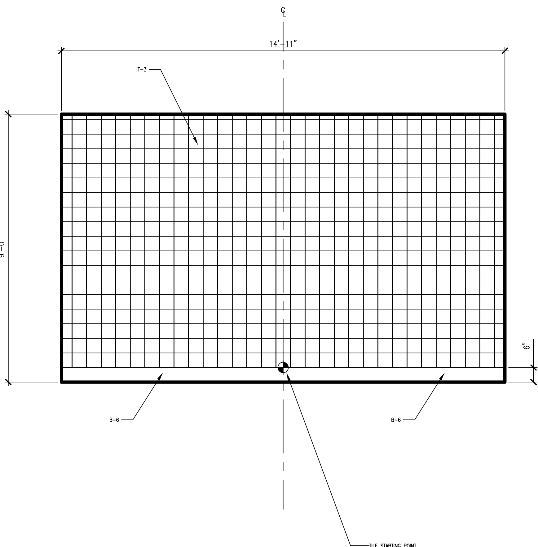
05 ELEVATION: SOUTH 1/2"=1'-0"
