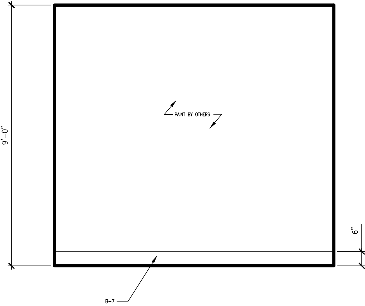
06 ELEVATION: SOUTH 1/2"=1'-0"
