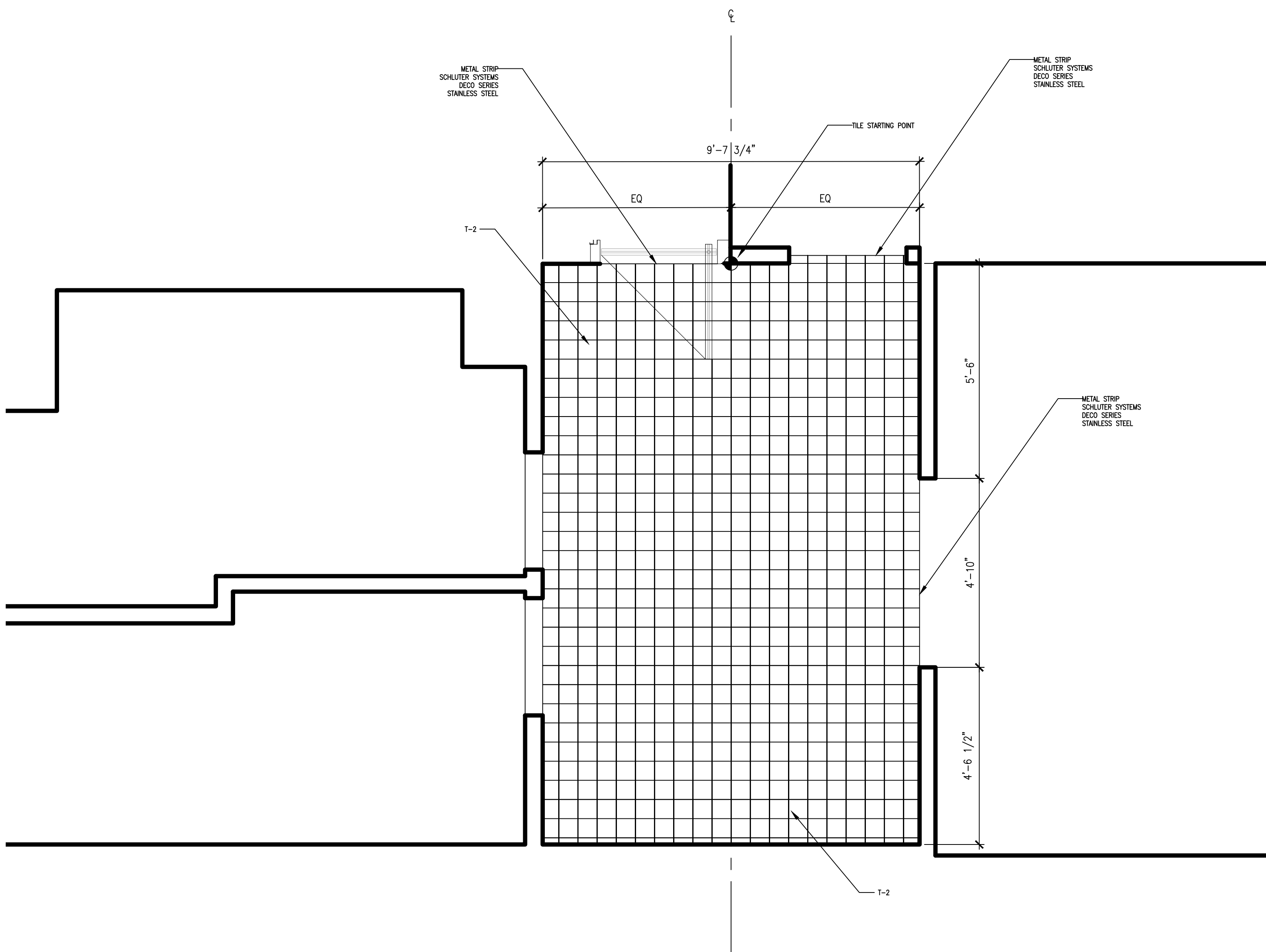
01 PLAN: SHOWROOM PANTRY 311 1/2"=1'-0"
