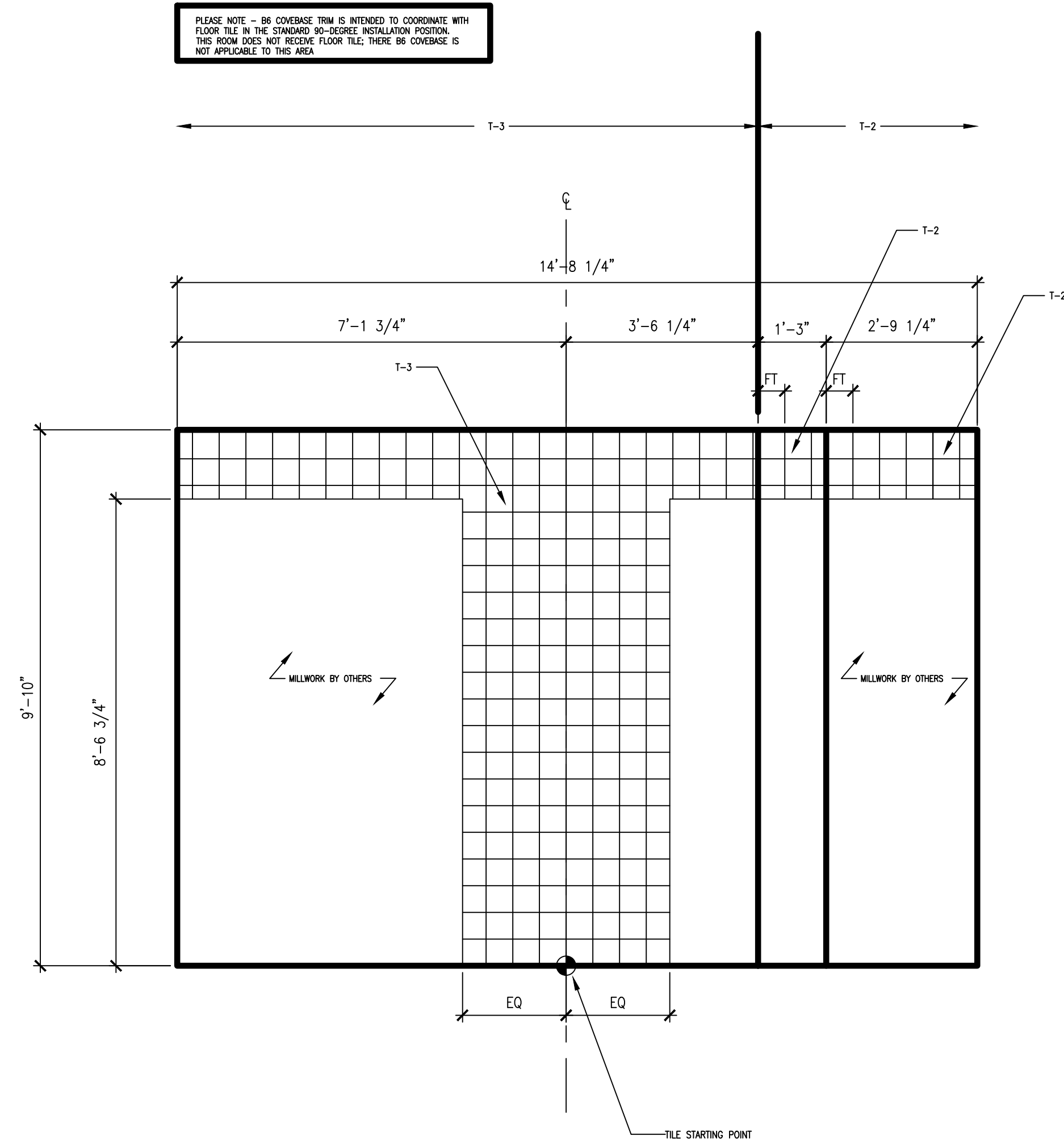
03 ELEVATION: EAST 1/2"=1'-0"
