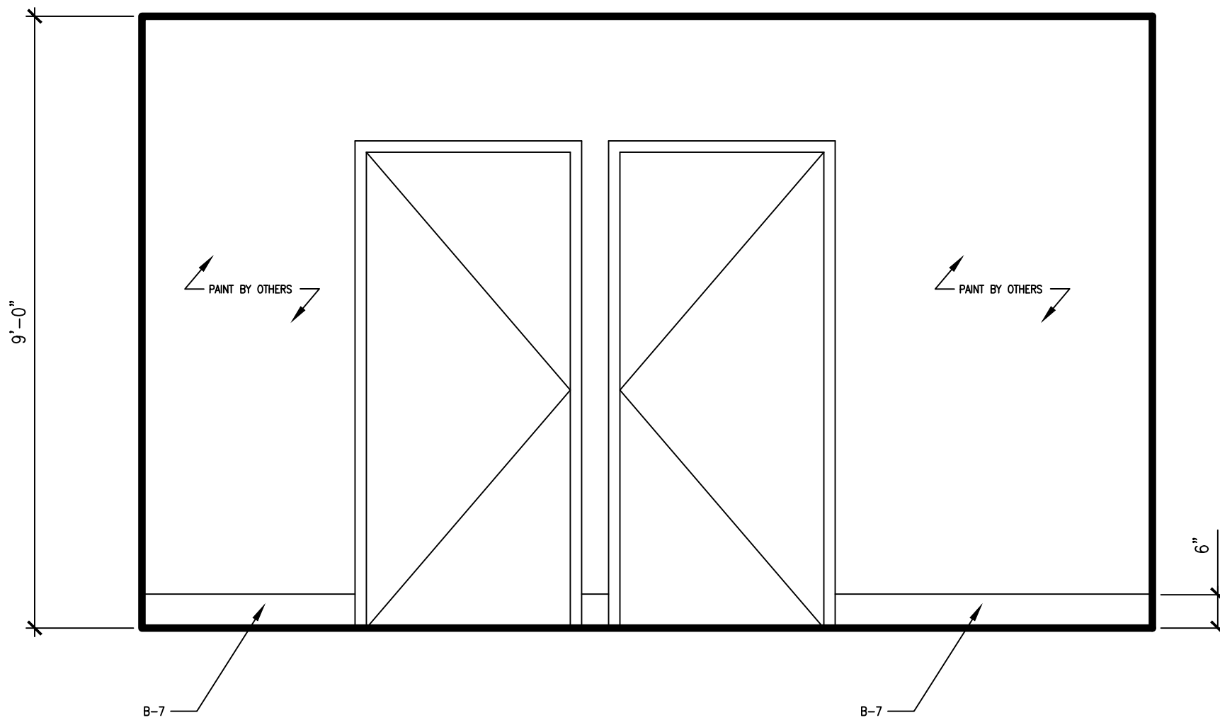
07 ELEVATION: WEST 1/2"=1'-0"
