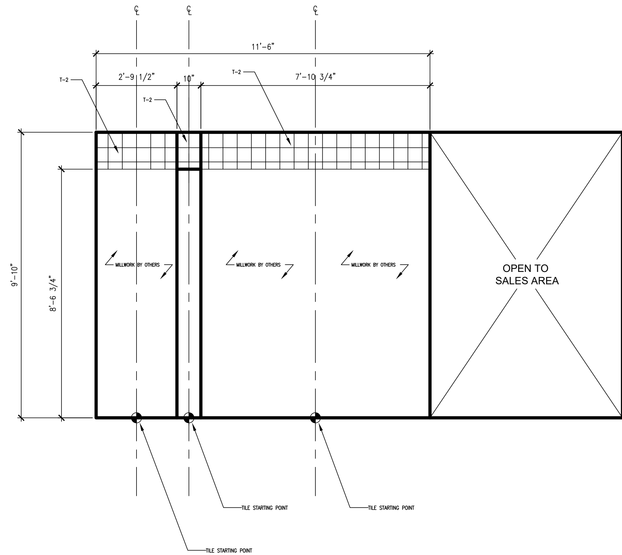
04 ELEVATION: SOUTH 1/2"=1'-0"
