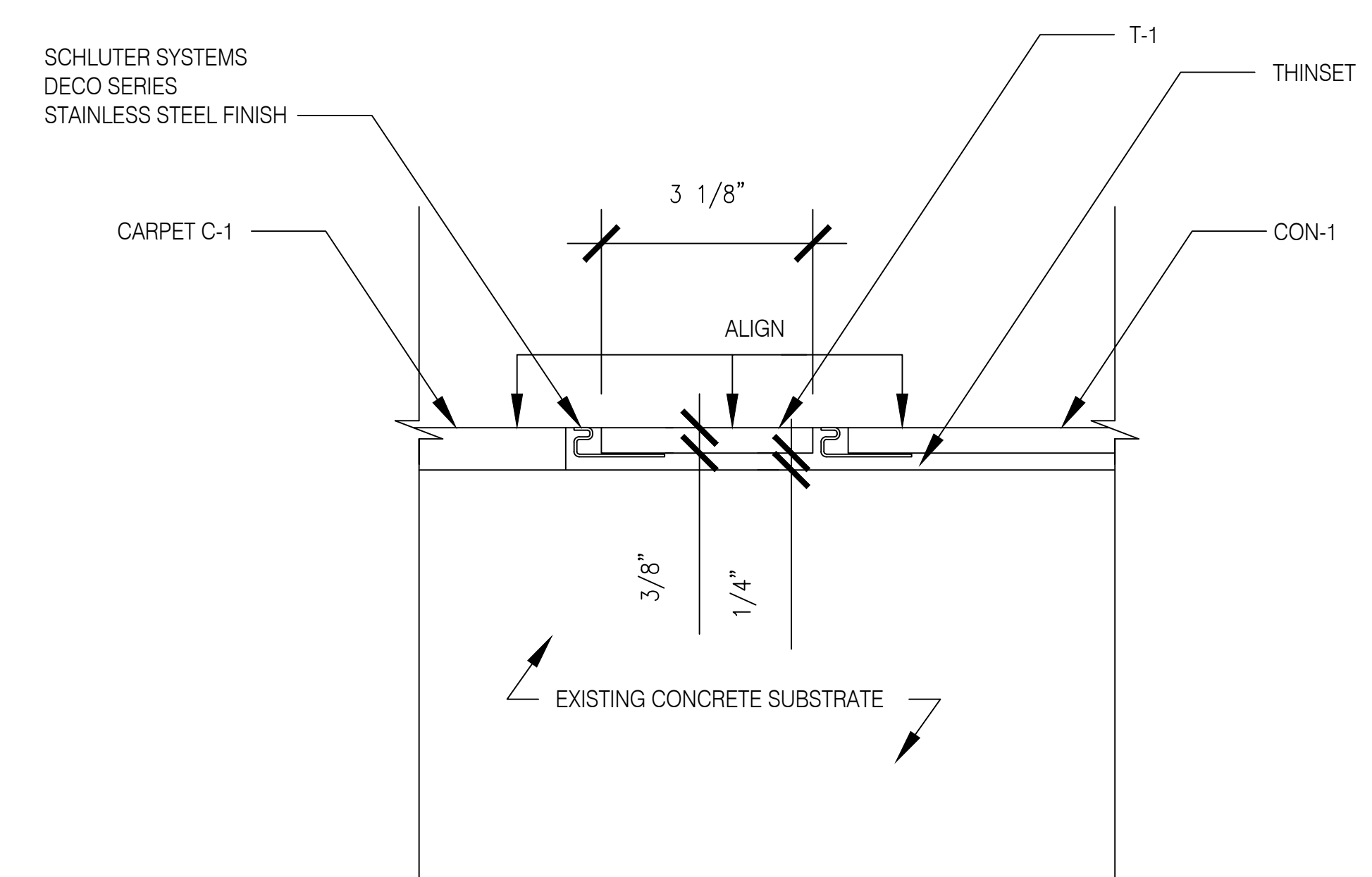
05 6'-1'-0" DETAIL: TILE/CARPET/CONCRETE TRANSITION AT SALES AREA 201
