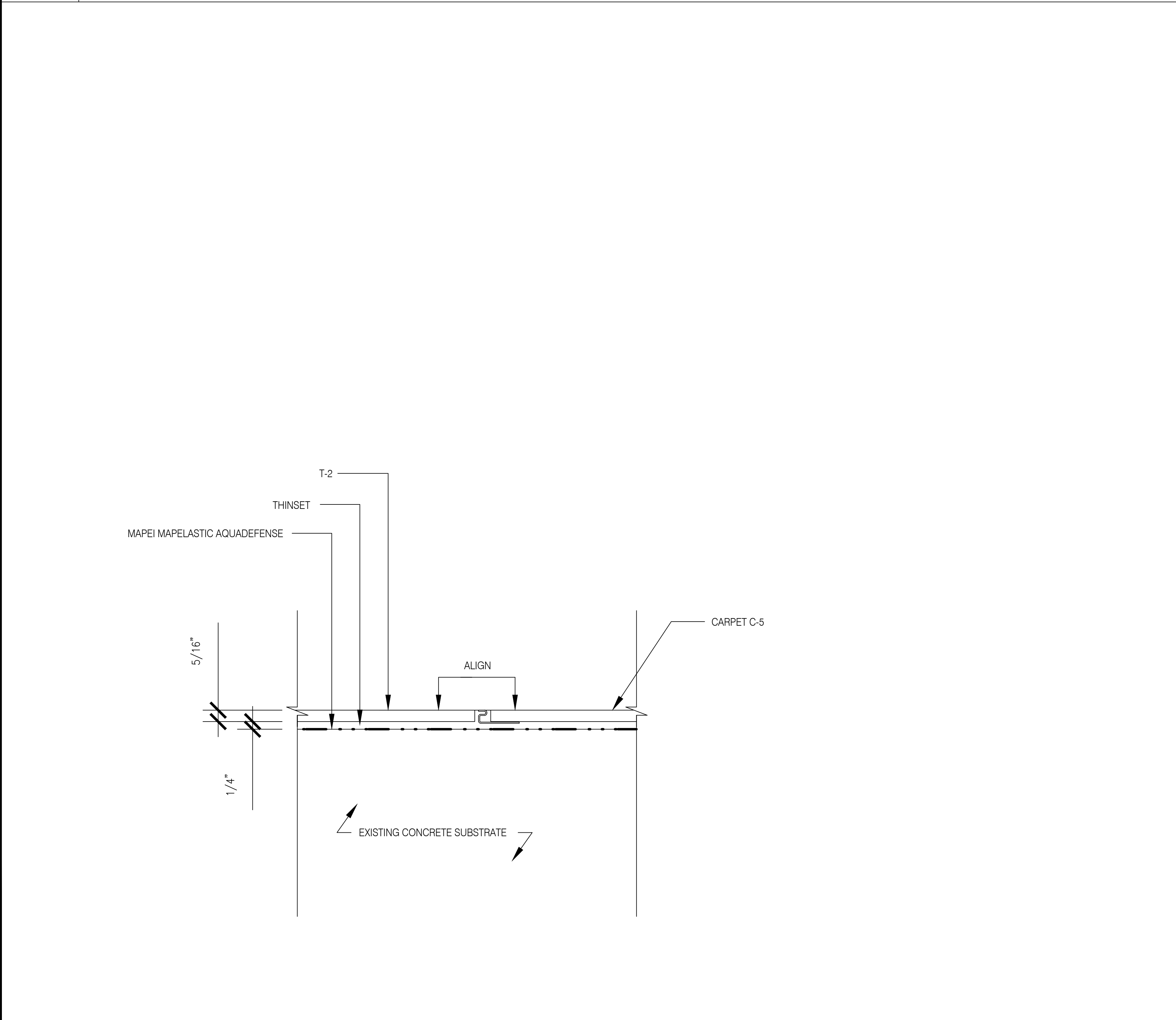
01 8" x 11" - 0" DETAIL: TILE/CARPET TRANSITION AT SHOWROOM PANTRY 311
