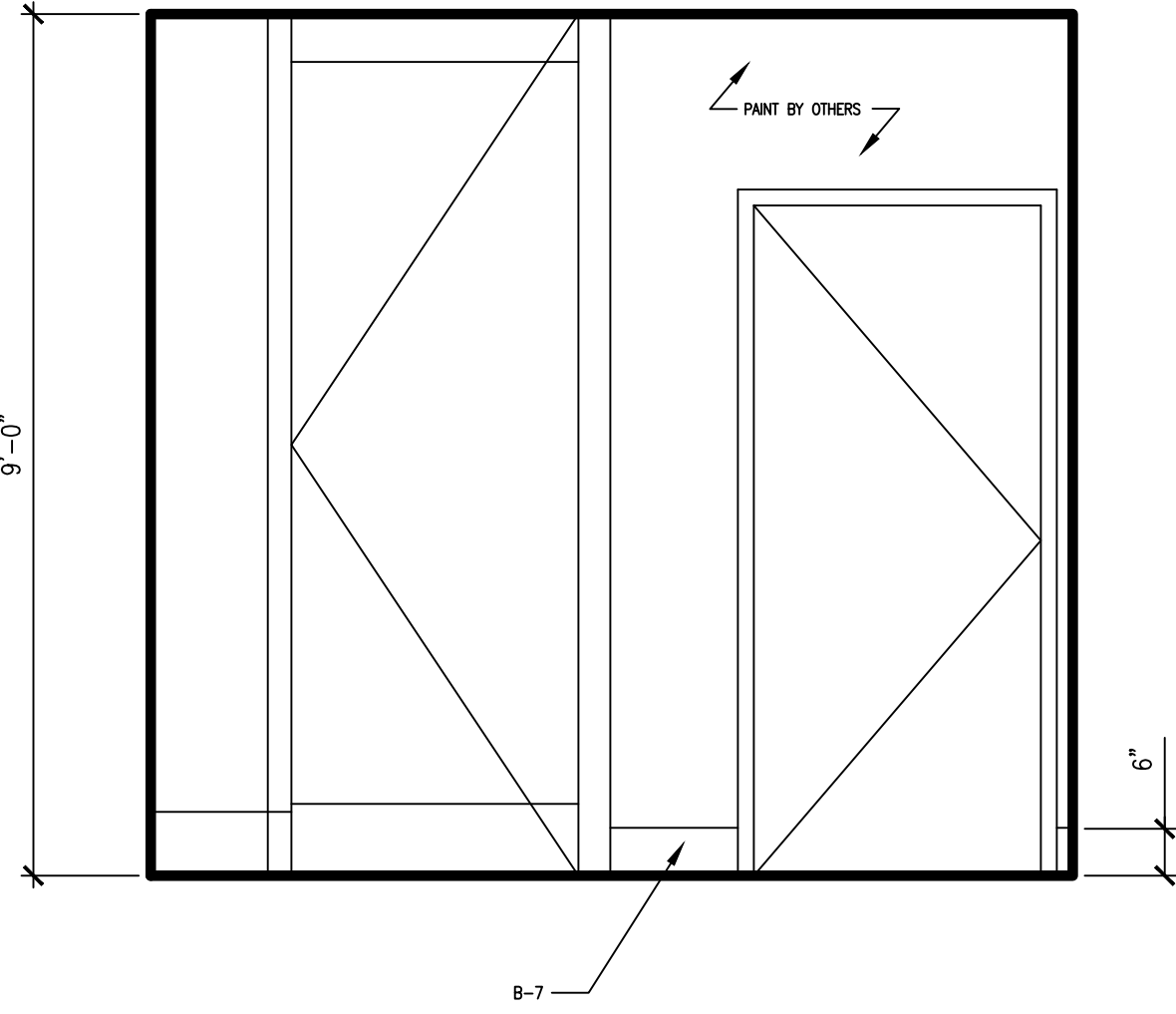
04 ELEVATION: NORTH 1/2"=1'-0"
