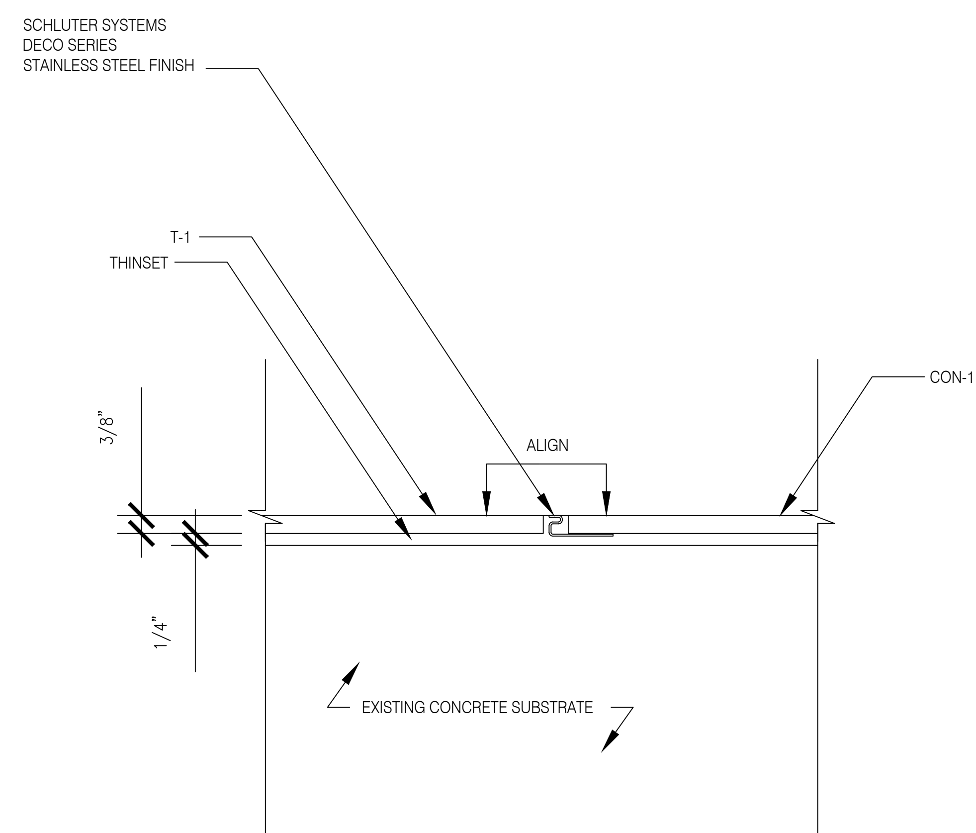
04 6"=1'-0" DETAIL: TILE/CONCRETE TRANSITION AT SALES AREA 201
