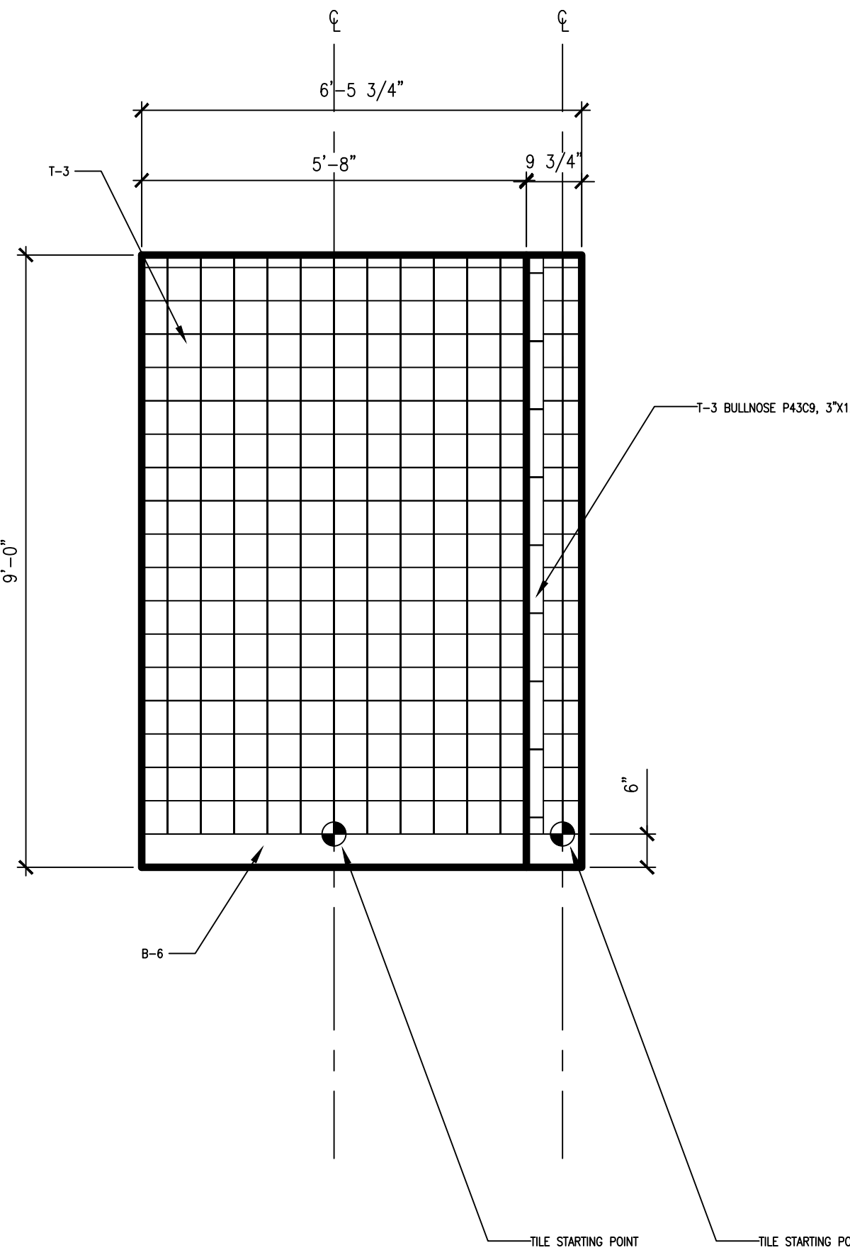
06 ELEVATION: WEST 1/2"=1'-0"
