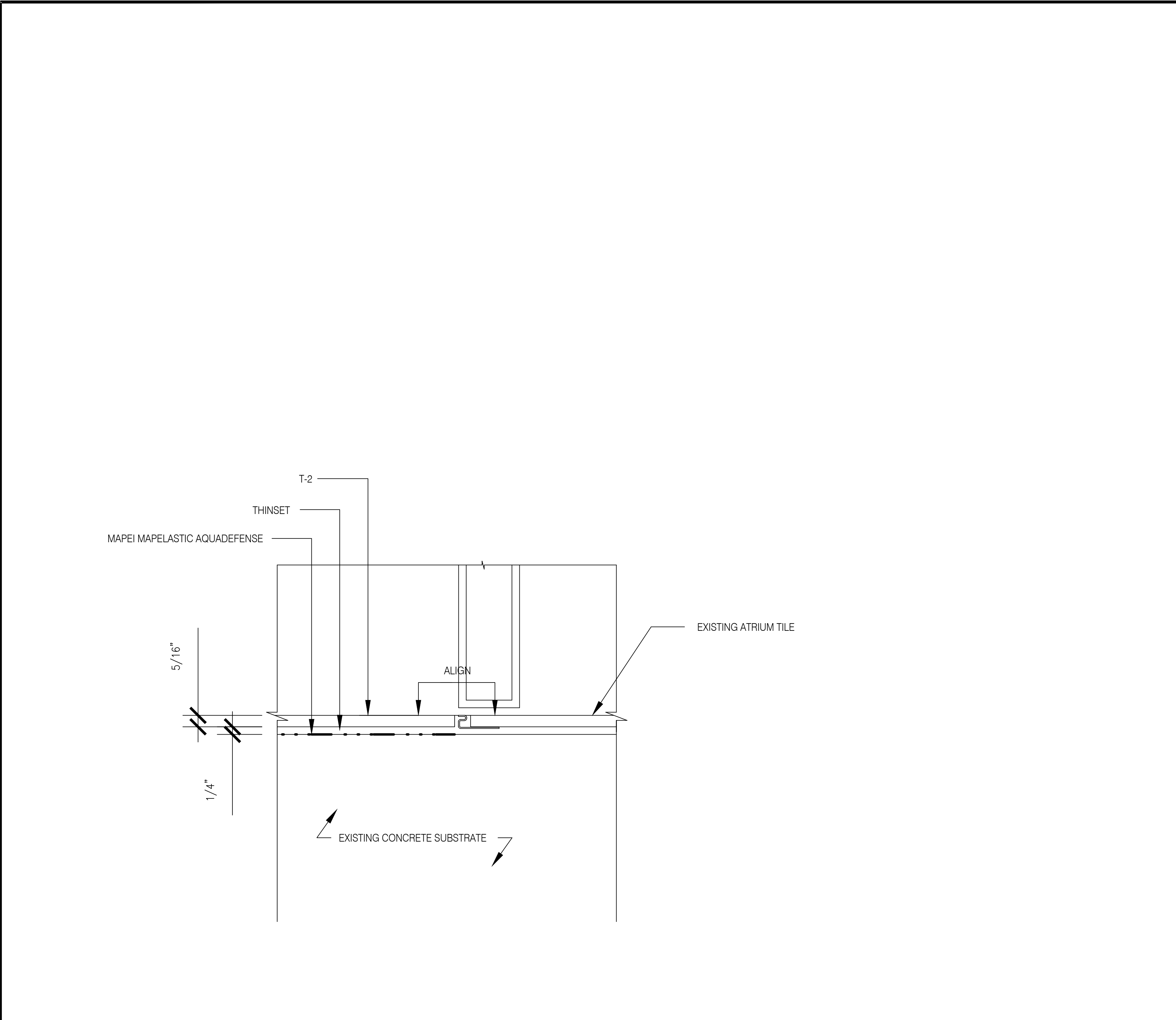
03 8" x 11" - 0" DETAIL: TILE/EXISTING FLOORING TRANSITION AT SHOWROOM PANTRY 311
