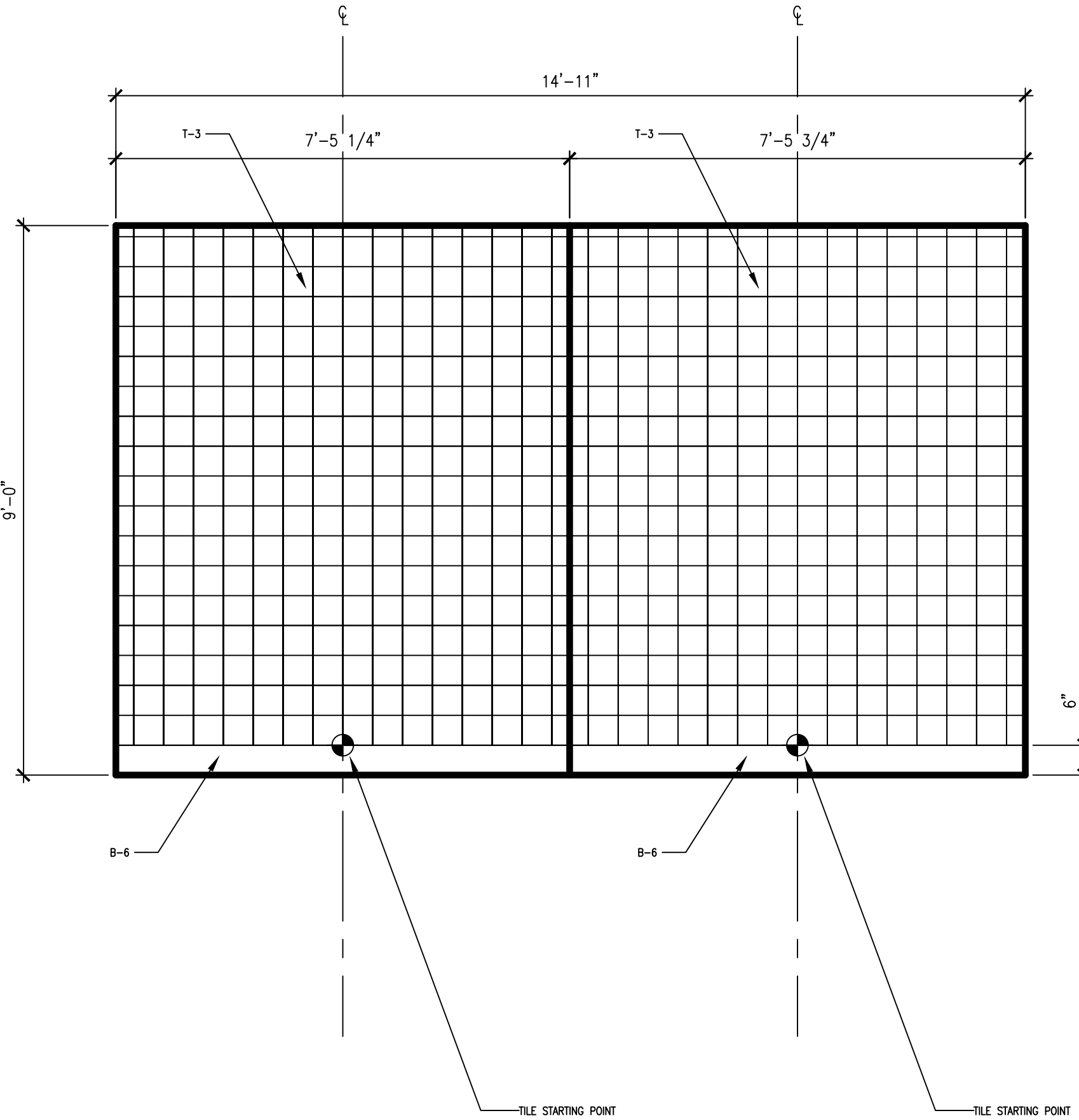
03 ELEVATION: NORTH 1/2"=1'-0"
