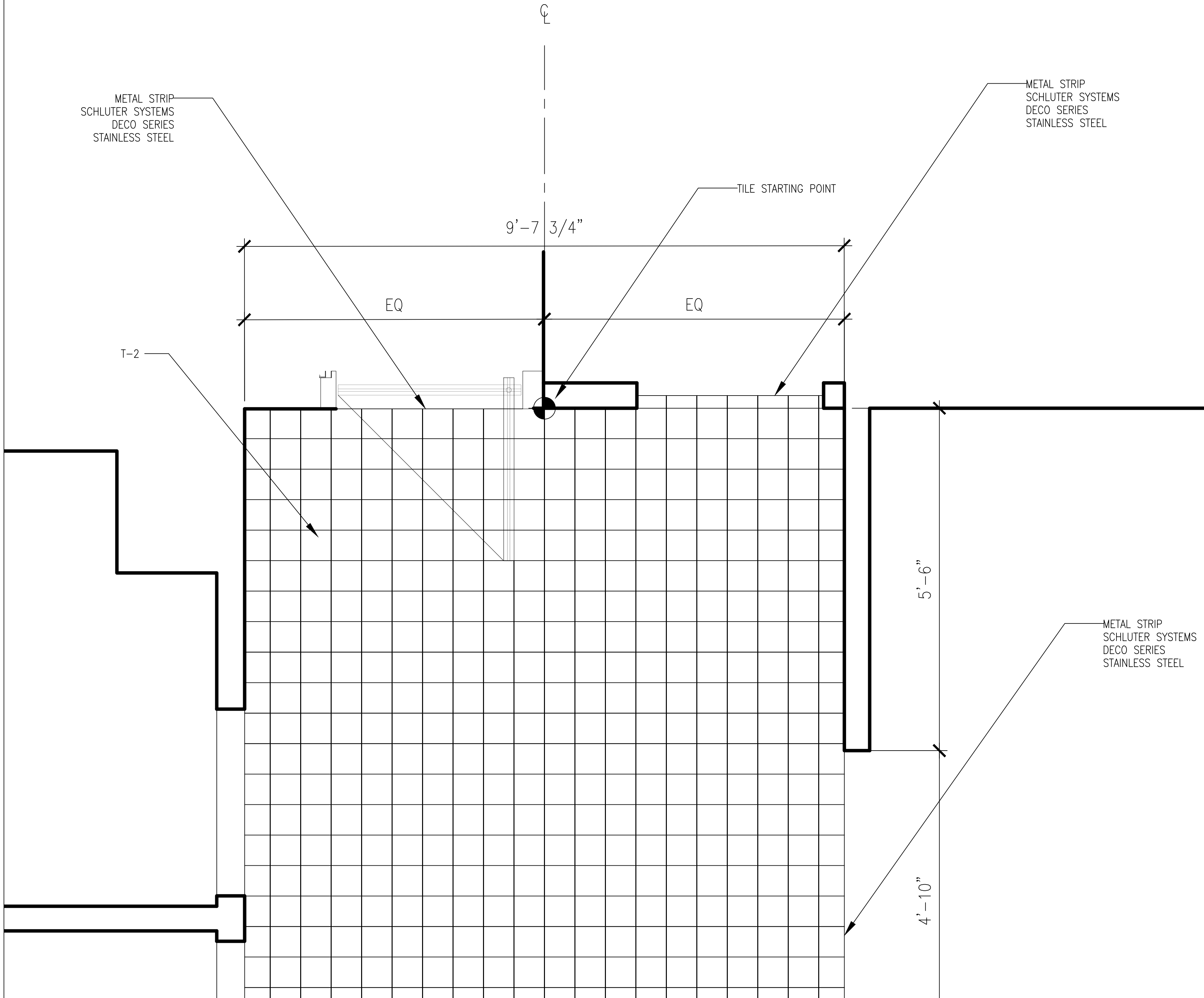
02 ENLARGED PLAN: SHOWROOM PANTRY 311 1/2"=1'-0"
